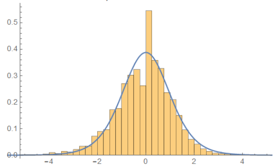
Simulation \frac{\bar{x} - \mu}{S/\sqrt{n}} , n=10, Poisson Data
