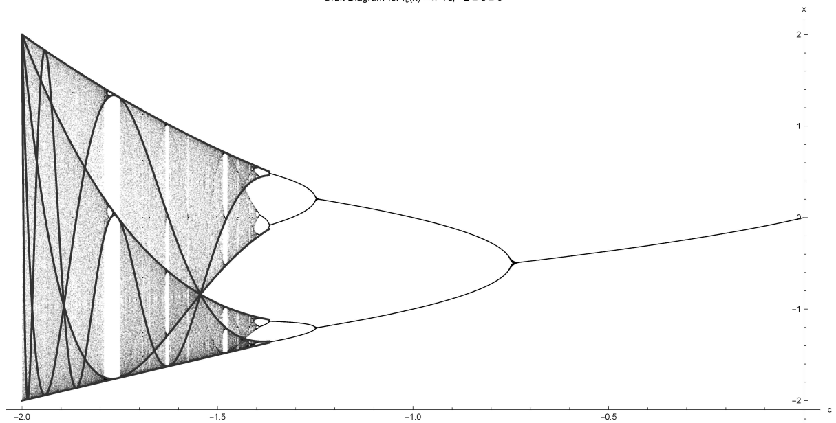
Orbit Diagram for f_c(x) = x^2 + c , -2 \leq c \leq 0
