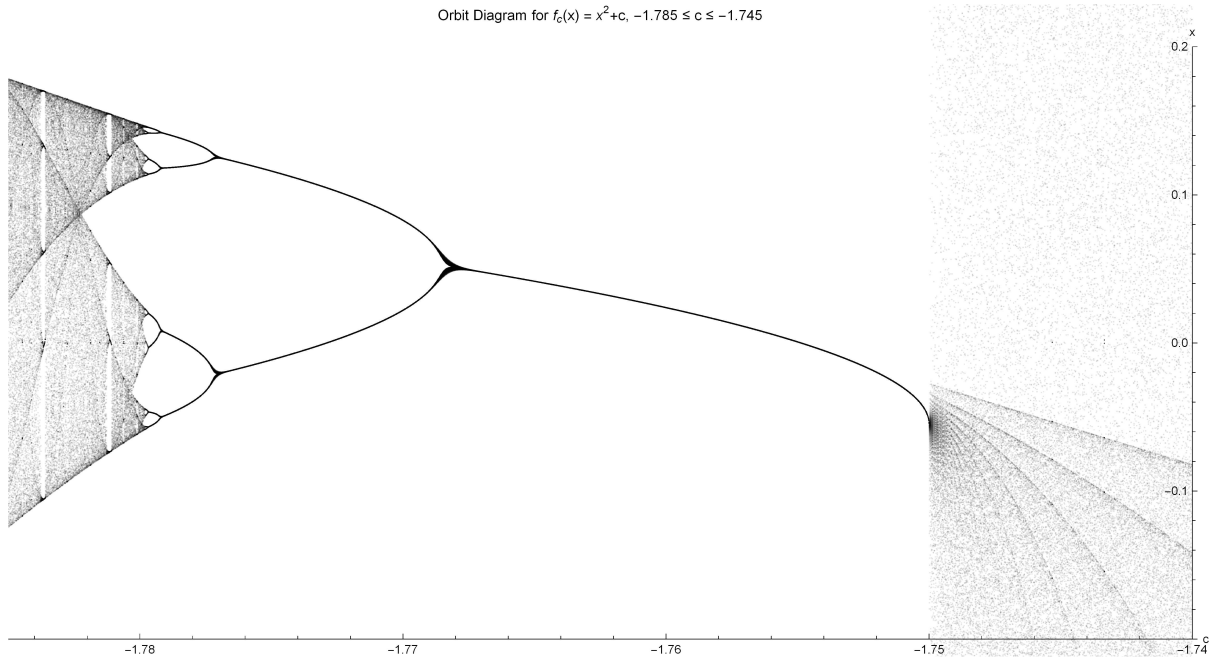
Orbit Diagram for f_c(x) = x^2 + c , -1.785 \leq c \leq -1.745
